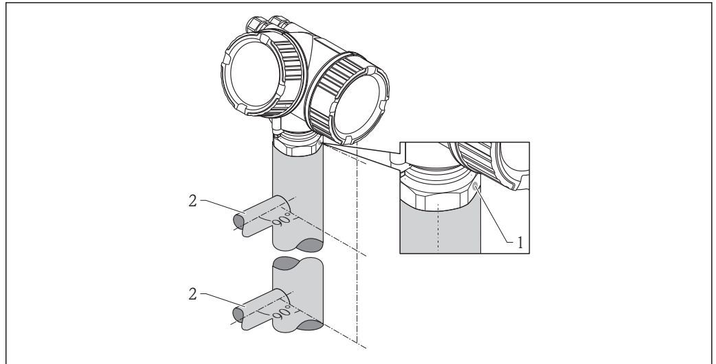
17 Installation in bypass
