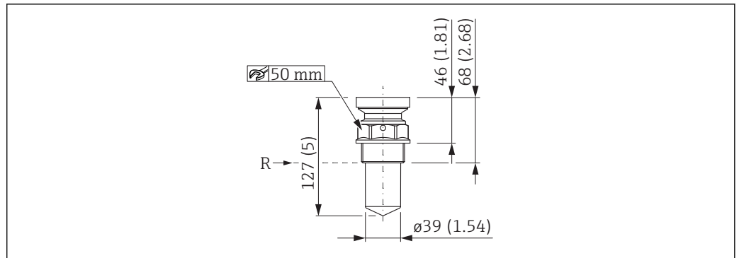
21 FMR50 with thread; dimensions: mm (in)
