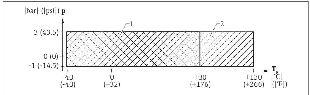
18 FMR50: Admissible range of process temperature and process pressure
