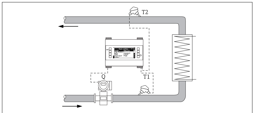
3 Calculation of the water heat quantity and water-heat differential from the input variables for flow ( Q ) and the temperature differential ( T1 - T2 )
