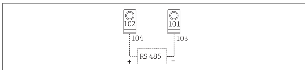
9 Interfaces RS485
