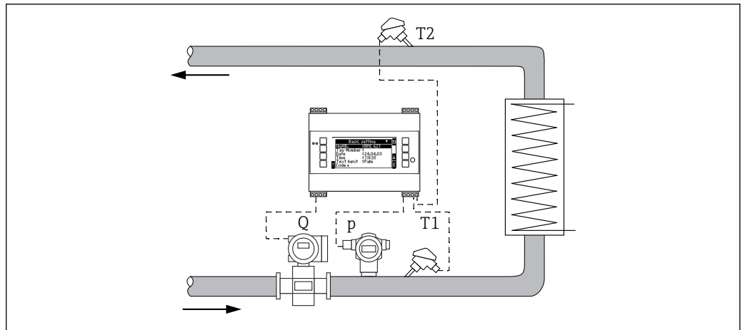
2 Calculation of the steam-heat differential and net steam quantity from the input variables for flow ( Q ), pressure ( p ) and the temperature differential ( T1 - T2 )
