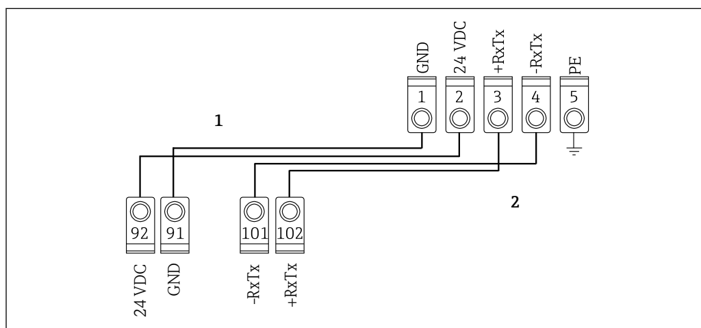
10 Connection of remote display and operating unit (option)
